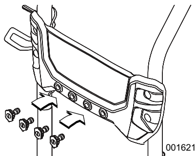
Figure 2-4. Insert Nozzles
